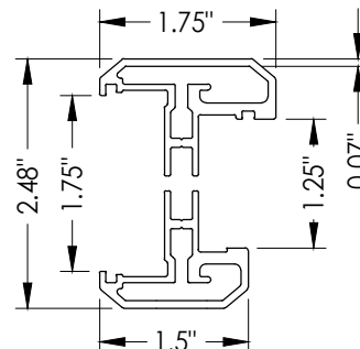
3B ODL FLAT ALUMINUM LITE FRAME 1-1/4" GLAZING
