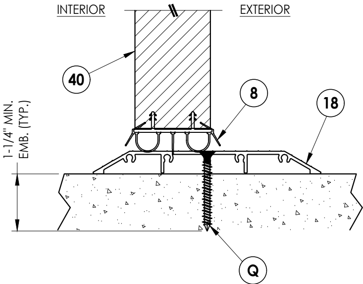
3 8 VERTICAL CROSS SECTION ADA Sill
