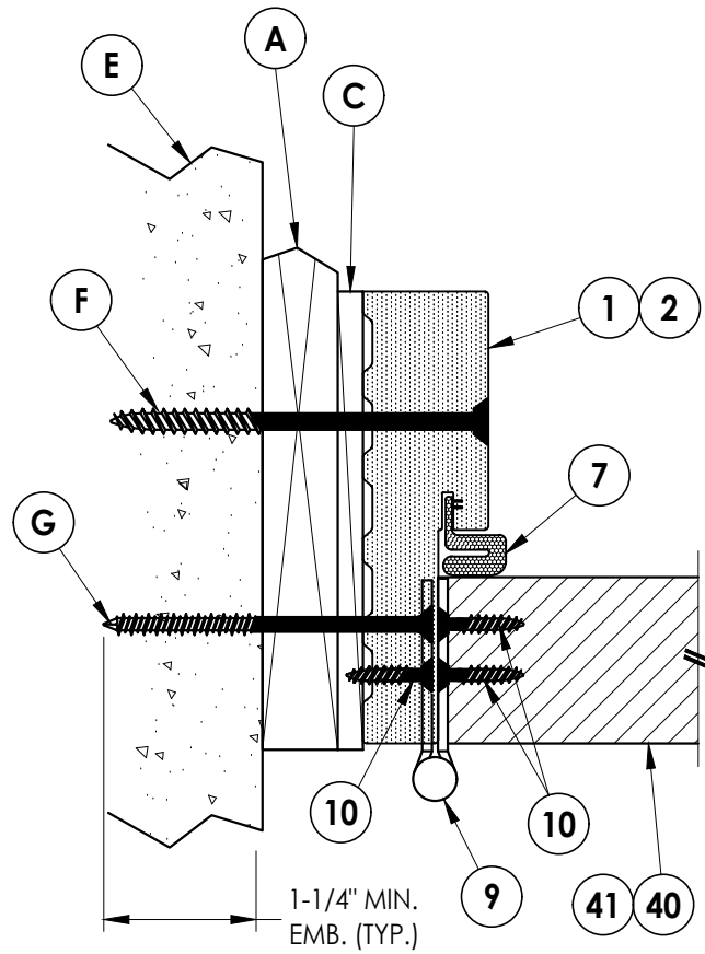
1 HORIZONTAL CROSS SECTION 6 Outswing Shown (Inswing Similar) Shown w/ 1X Buck
