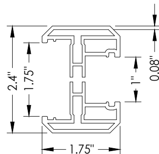
3A ODL FLAT ALUMINUM LITE FRAME 1" GLAZING
