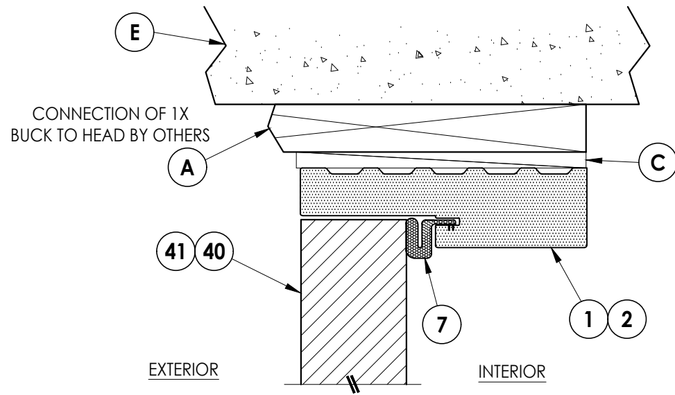
3 VERTICAL CROSS SECTION 6 Outswing Shown (Inswing Similar) Shown w/ 1X Buck
