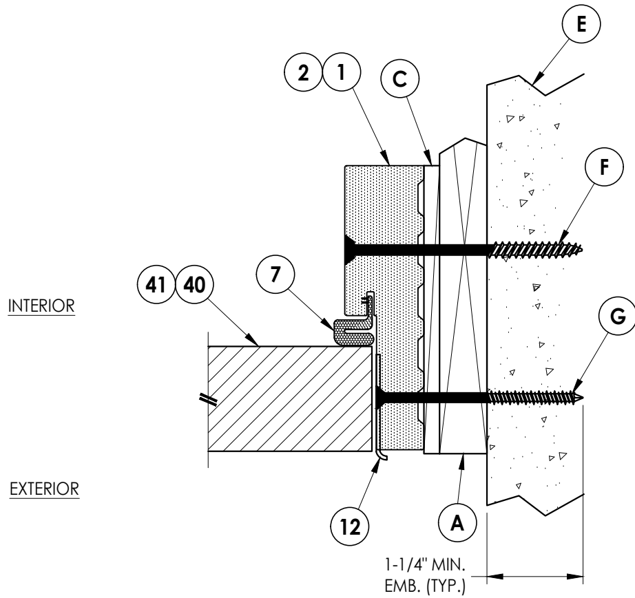
2 HORIZONTAL CROSS SECTION 6 Outswing Shown (Inswing Similar) Shown w/ 1X Buck
